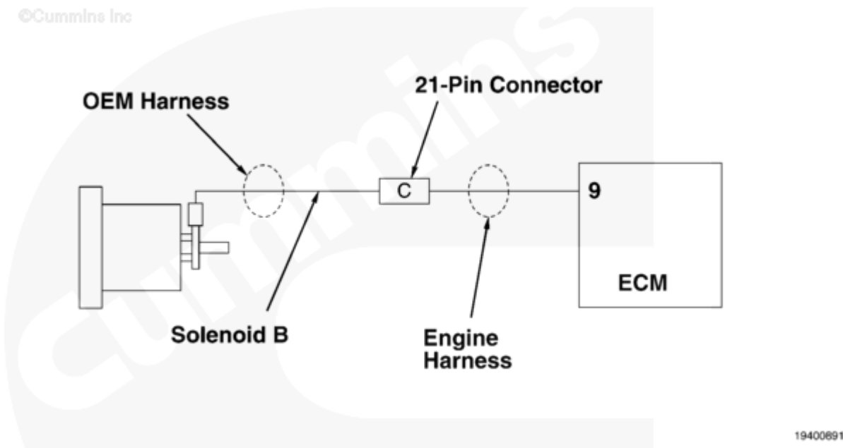
Solenoid B Circuit
