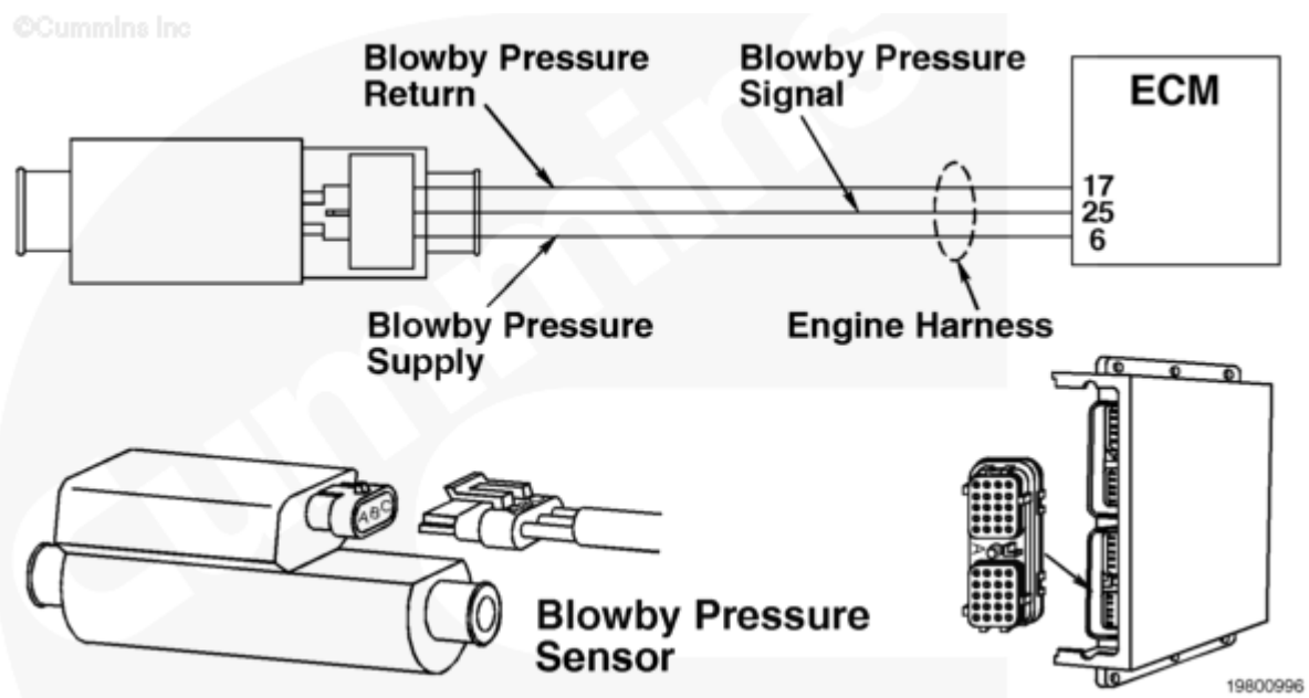
Blowby Pressure Sensor Circuit
