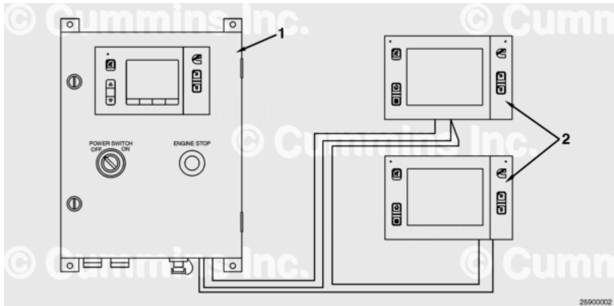
C Command HD Elite Marine Panel System PS106 & C Command HD Elite Marine Panel System PS107
