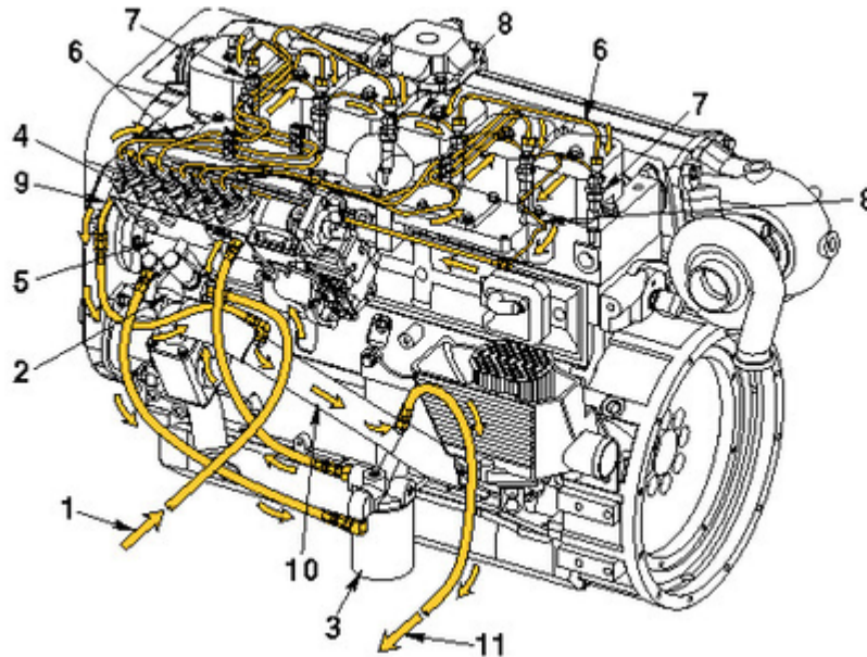
Six Cylinder Fuel System
