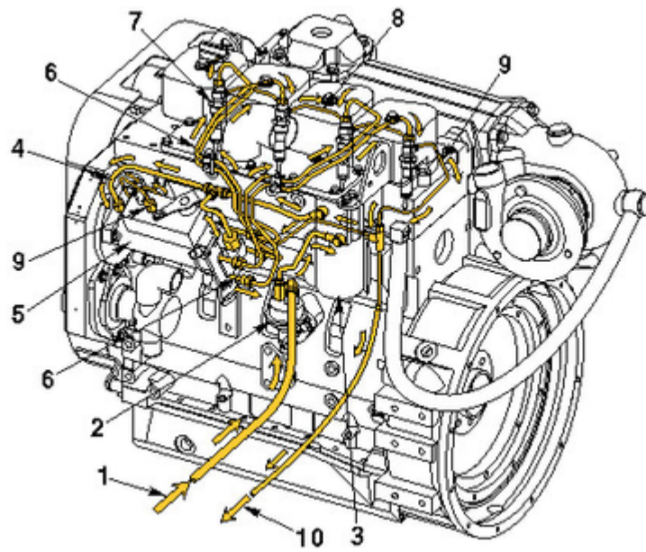
Four Cylinder Fuel System
