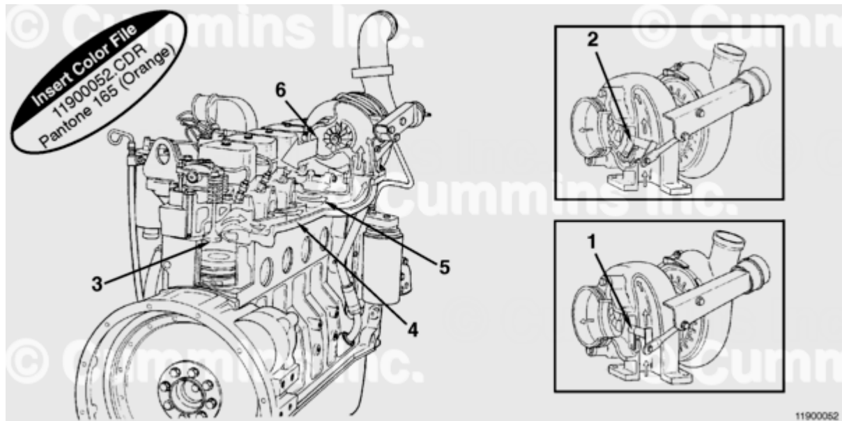
Turbocharged with Wastegate
