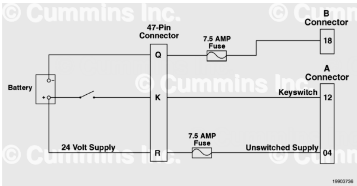
Power Supply Circuit
