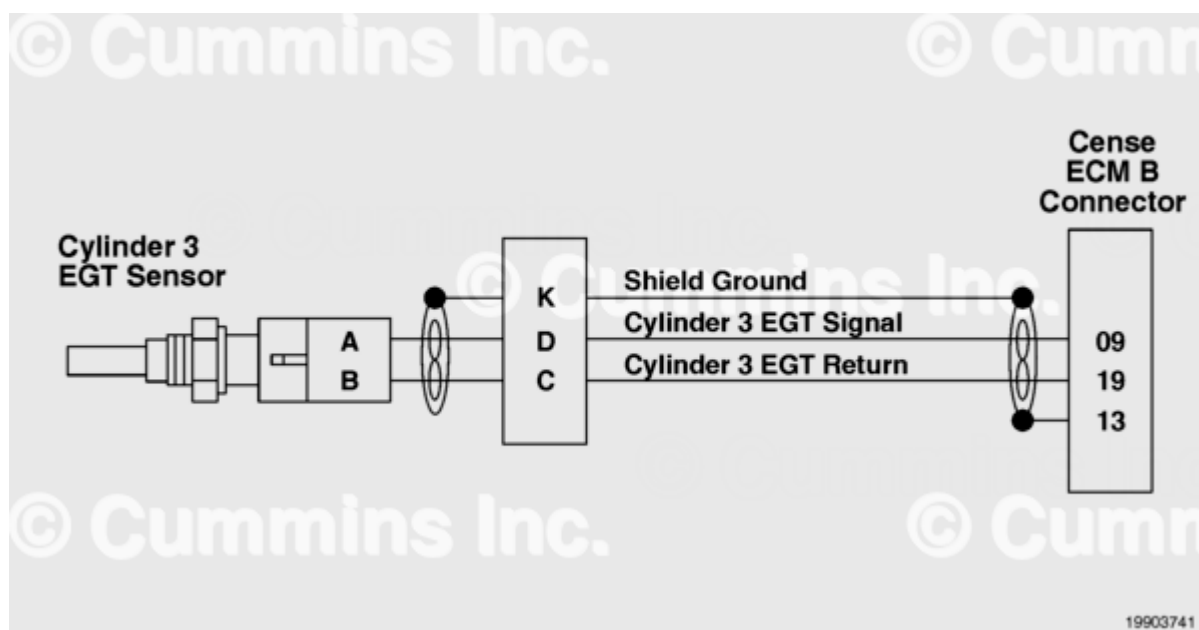
Exhaust Gas Temperature Sensor Circuit Cylinder 3
