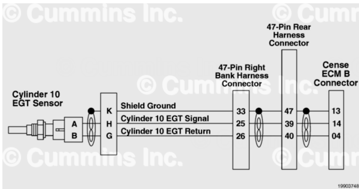
Exhaust Gas Temperature Sensor Circuit Cylinder 10
