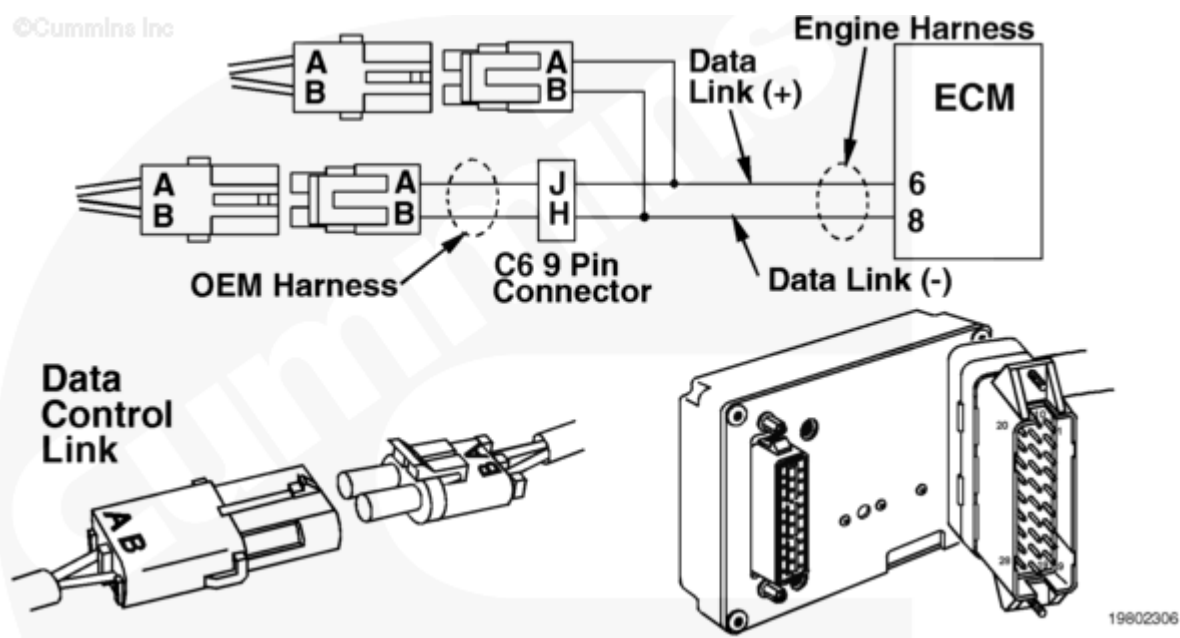
Datalink Circuit
