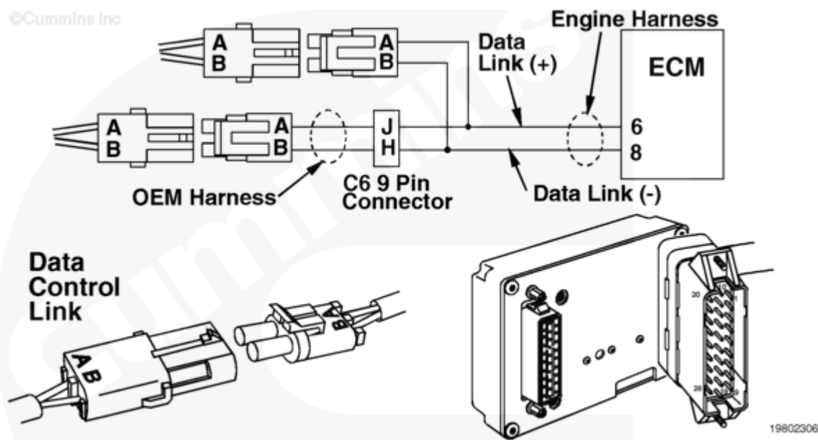
Datalink Circuit
