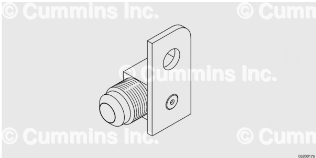
Figure 2: New fuel return bracket, Part Number 4985465.
