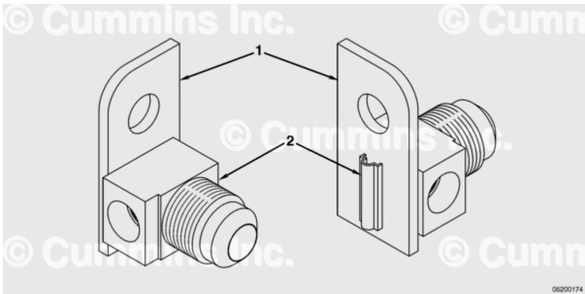
Figure 1: Old fuel return bracket, Part Number 3401236.
