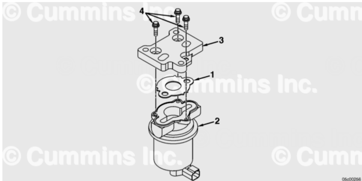
Figure 1, Fuel Transfer Pump Assembly - (1) Gasket, (2) Fuel Transfer Pump, (3) Mounting Support, 4) Capscrew
