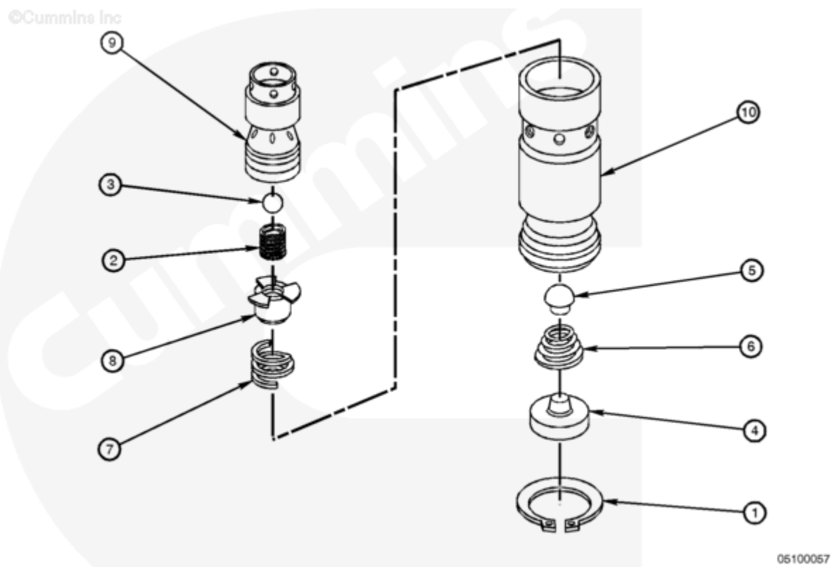
Figure 8. Current STC Injector Tappet Parts
