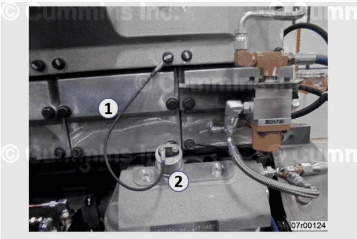
Figure 1, New Ground Wire and Transducer Installed.
