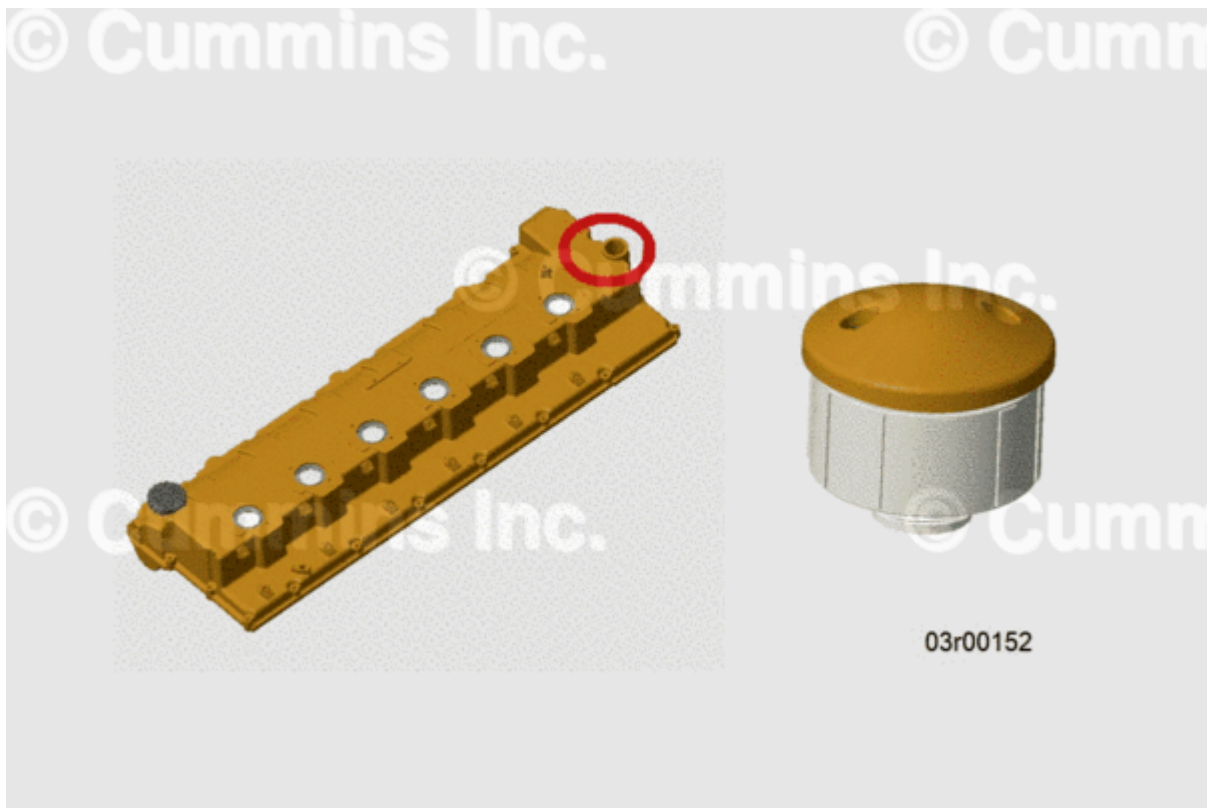
Figure 1, Rocker Lever Cover, Pressure Relief Valve, and Pressure Relief Valve Location.
