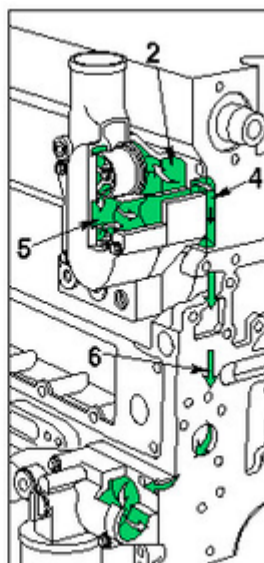
Dual Thermostat
