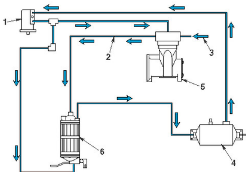
WABCO - Type System with Air Dryer
