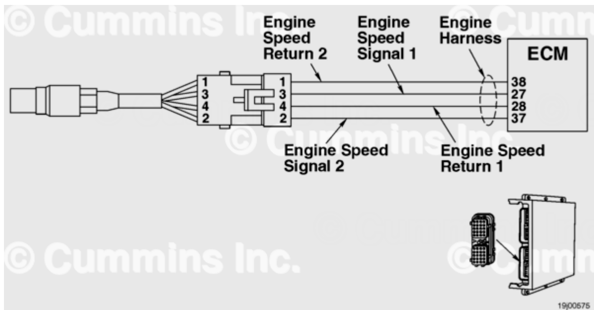
Engine Speed Sensor Circuit
