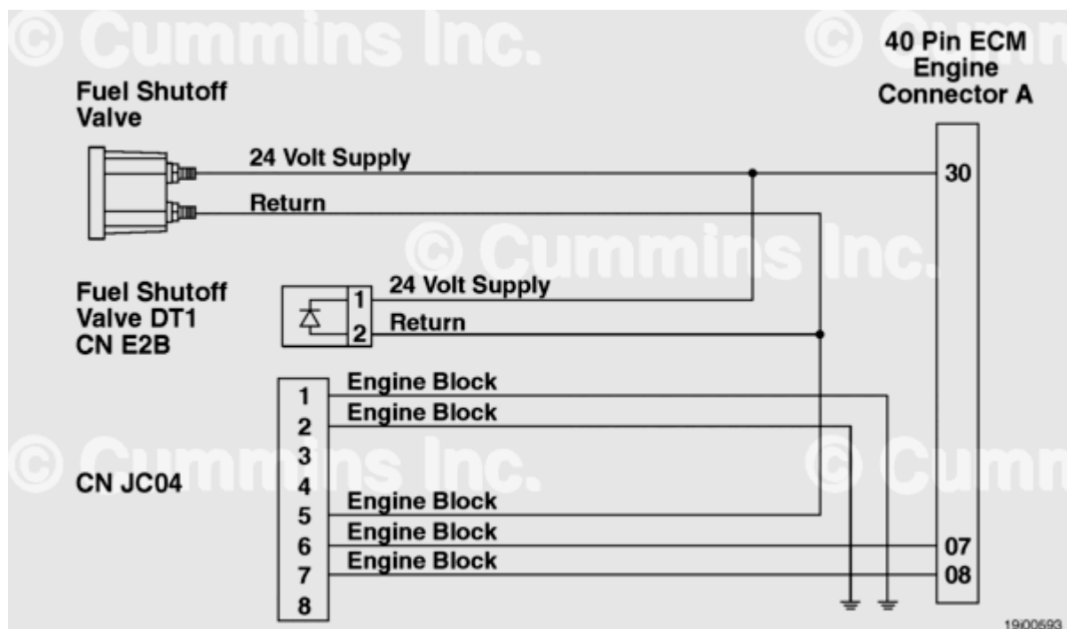
QSK23 - Fuel Shutoff Solenoid Circuit
