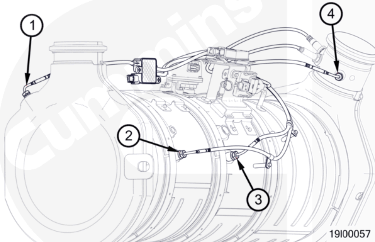
Figure 2, Aftertreatment Exhaust Gas Temperature Sensor Probe Locations.
