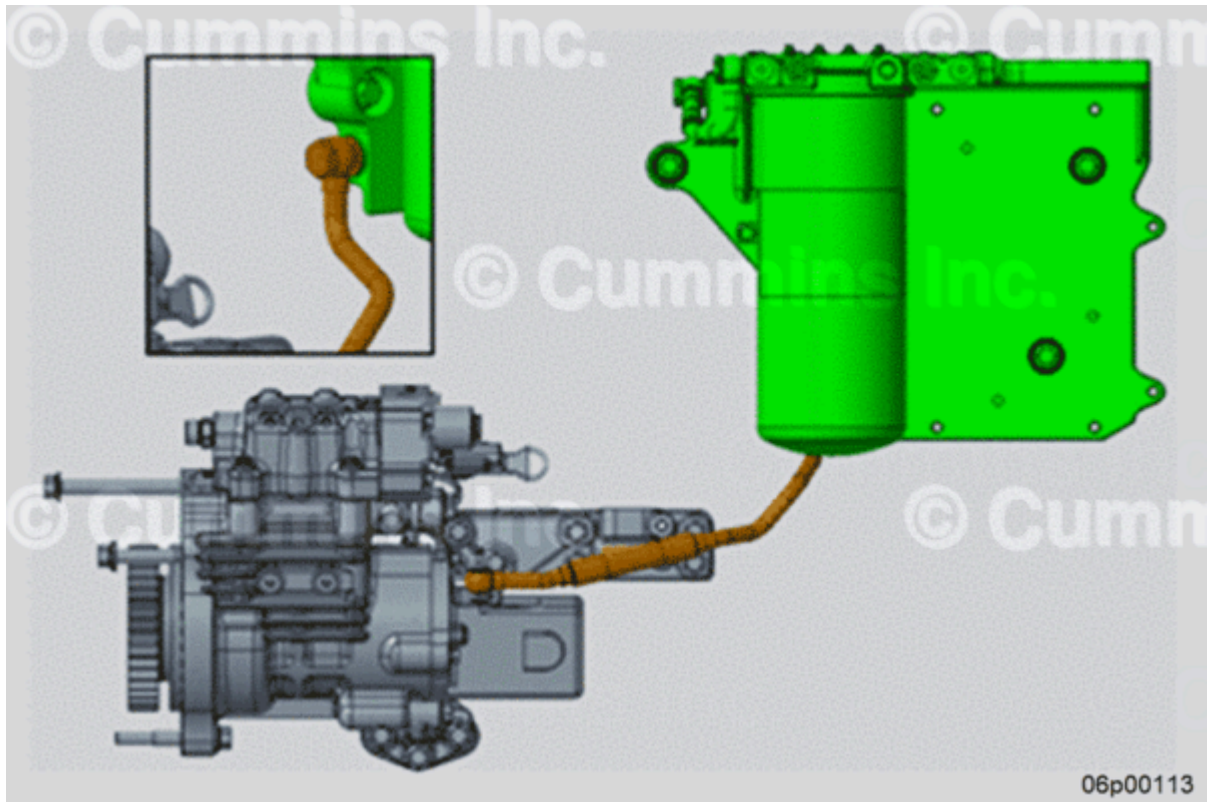
Figure 9, Existing Outlet Line Part Number 3688317 (Brown), Existing Gear Pump Part Number 4307482 (Gray), Fuel Filter Arrangement Part Number 3685850 (Green).
