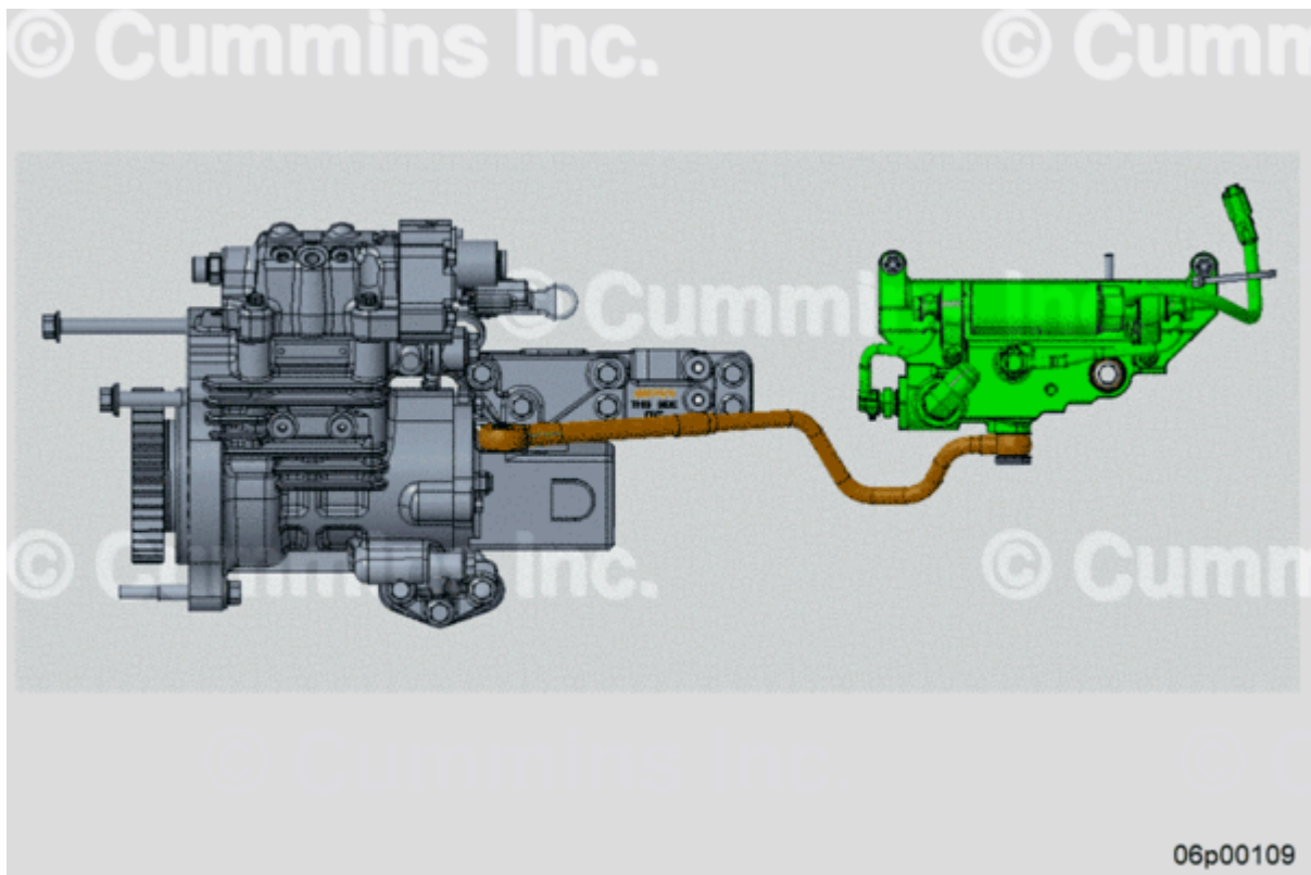
Figure 5, Existing Inlet Line Part Number 3689169 (Brown), Existing Gear Pump Part Number 4307482 (Gray), Priming Pump Part Number 3688896 (Green).
