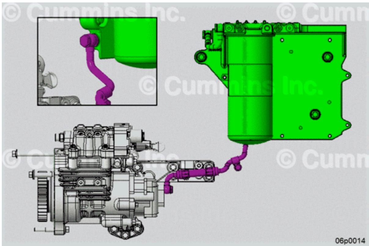
Figure 10, New Outlet Line Part Number 5575372 (Purple), New Gear Pump Part Number 5491782 (White), Fuel Filter Arrangement Part Number 3685850 (Green).
