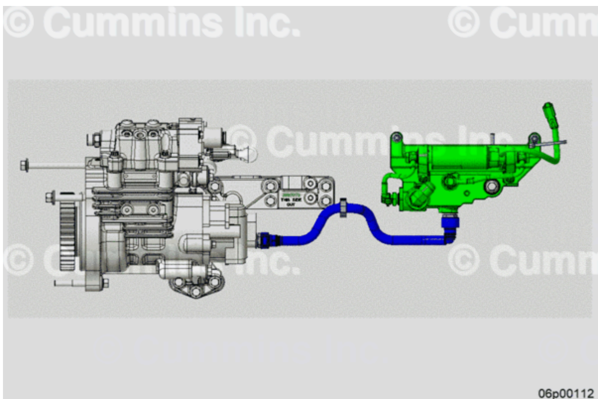
Figure 8, New Inlet Line Part Number 5481207 (Blue), New Gear Pump Part Number 5491782 (White), Priming Pump Part Number 3688896 (Green).
