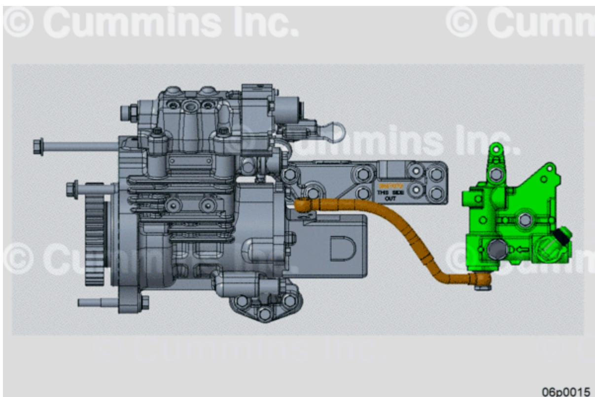
Figure 11, Existing Outlet Line Part Number 3688112 (Brown), Existing Gear Pump Part Number 4307482 (Gray), Priming Pump Part Number 3692468 (Green).
