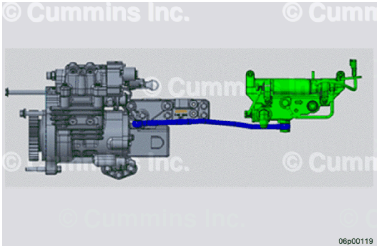
Figure 17, Existing Inlet Line Part Number 5481051 (Blue), Existing Gear Pump Part Number 4307482 (Gray), Priming Pump Part Number 5481052 (Green).
