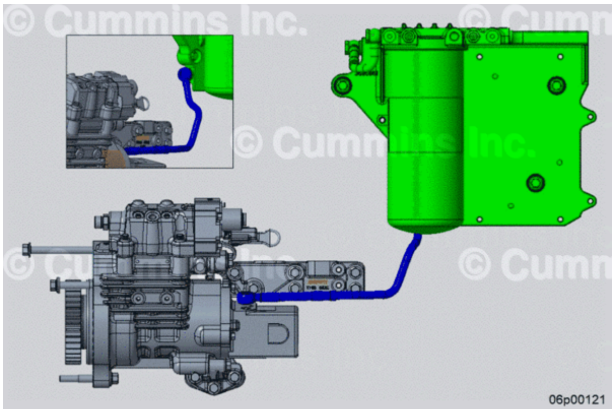
Figure 19, Existing Outlet Line Part Number 5481055 (Blue), Existing Gear Pump Part Number 4307482 (Gray), Fuel Filter Arrangement Part Number 3685850 (Green).
