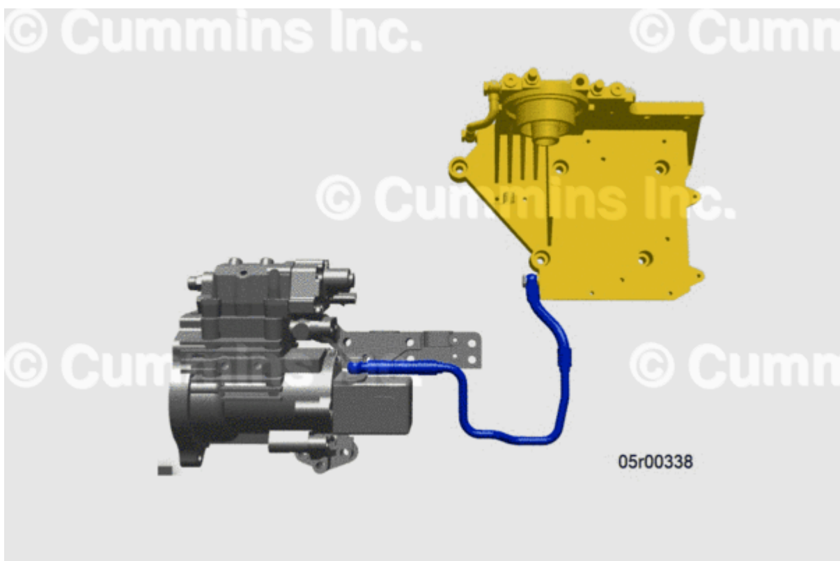
Figure 15, Existing Outlet Line, Part Number 3688398 (Blue), Existing Gear Pump, Part Number 4307482 (Grey), Fuel Filter Arrangement, Part Number 3685850 (Yellow).
