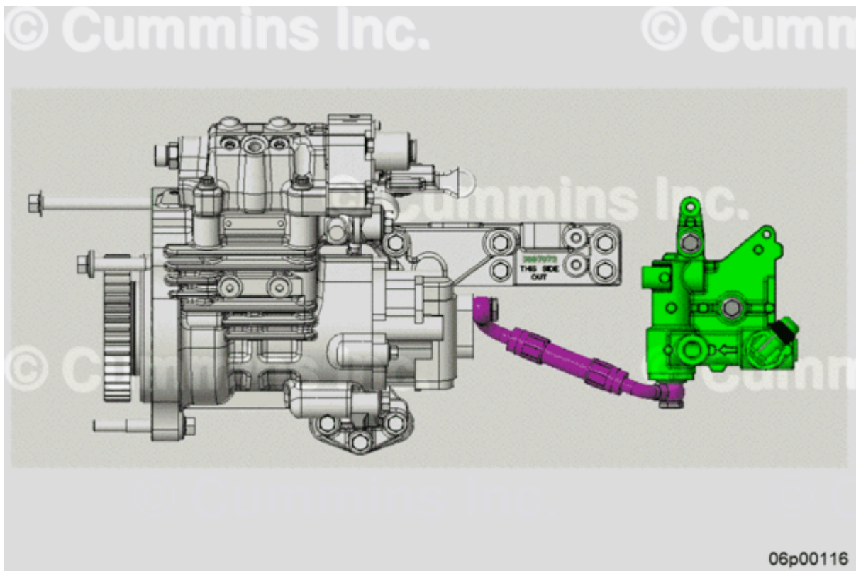
Figure 12, New Outlet Line Part Number 5575371 (Purple), New Gear Pump Part Number 5491782 (White), Priming Pump Part Number 3692468 (Green).
