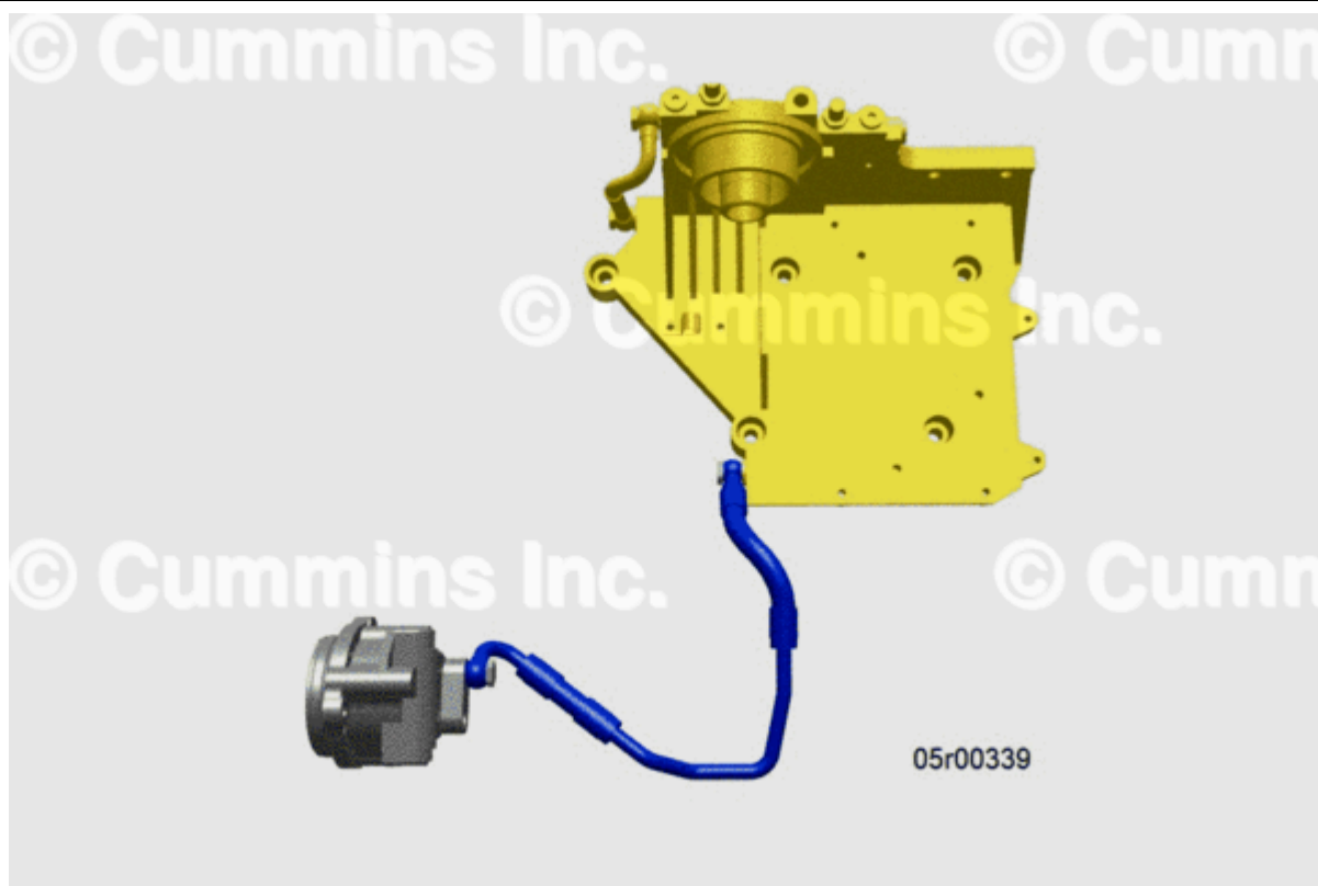
Figure 16, New Outlet Line, Part Number 5575373 (Blue), New Gear Pump Part Number 5491782 (Grey), Fuel Filter Arrangement, Part Number 3685850 (Yellow).
