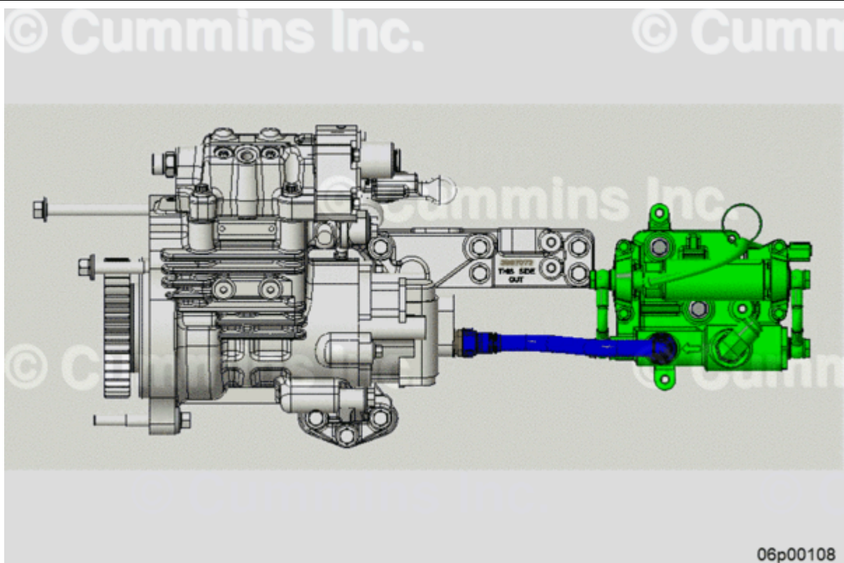
Figure 4, New Inlet Line Part Number 5481205 (Blue), New Gear Pump Part Number 5491782 (White), Priming Pump Part Number 3692468 (Green).
