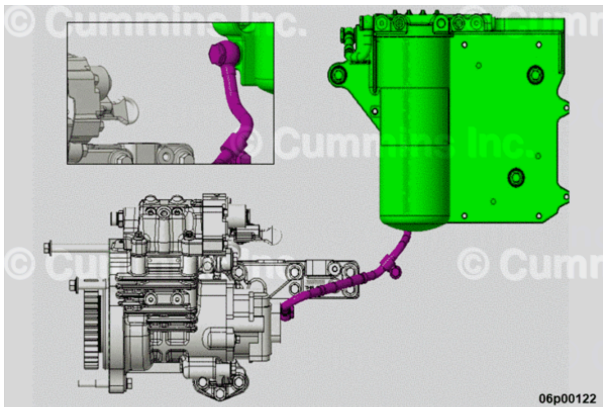
Figure 20, New Outlet Line Part Number 5566482 (Purple), New Gear Pump Part Number 5491782 (White), Fuel Filter Arrangement Part Number 3685850 (Green).
