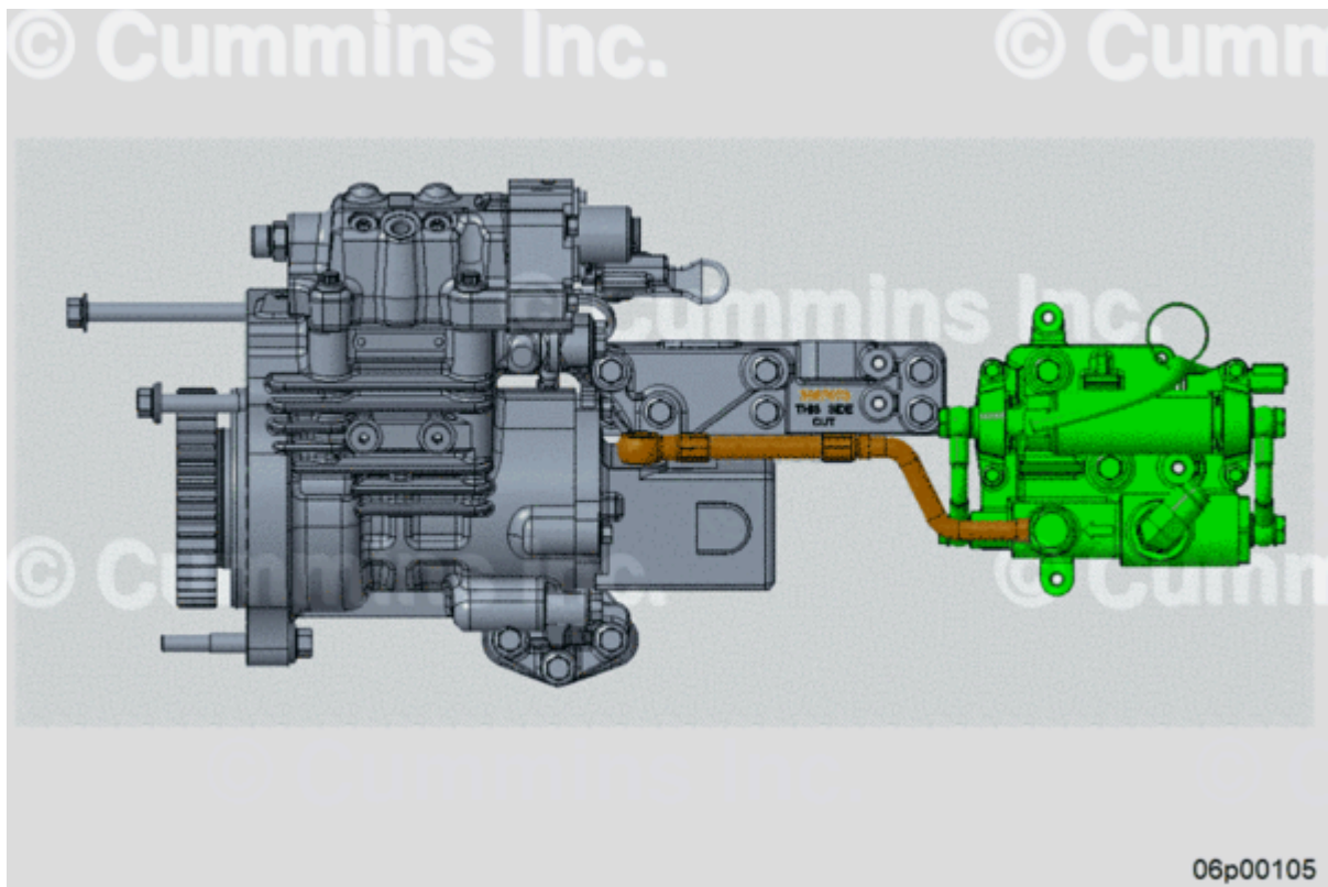
Figure 1, Existing Inlet Line Part Number 3688089 (Brown), Existing Gear Pump Part Number 4307482 (Gray), Priming Pump Part Number 3692468 (Green).
