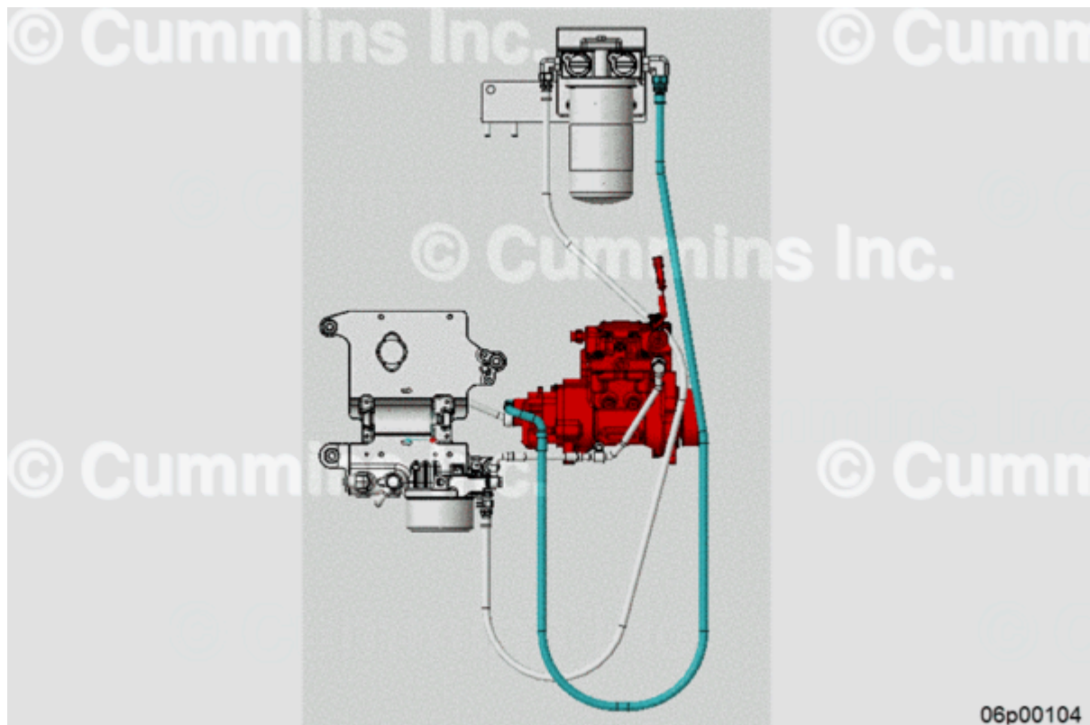
Figure 26, New Outlet Line, Part Number 5479013 (Teal), New Gear Pump, Part Number 5491783 (Red), Fuel Filter Arrangement (White)
