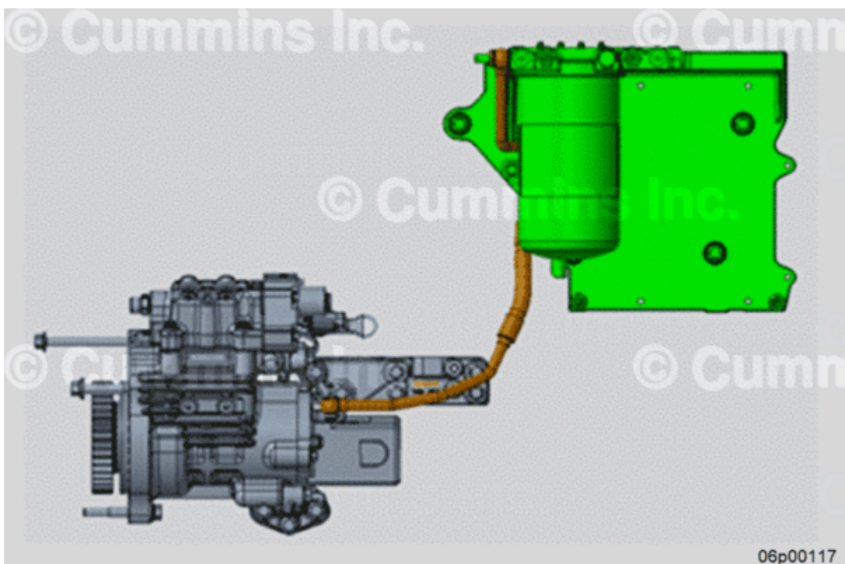
Figure 13, Existing Outlet Line Part Number 5558764 (Brown), Existing Gear Pump Part Number 4307482 (Gray), Fuel Filter Arrangement Part Number 3685850 (Green).
