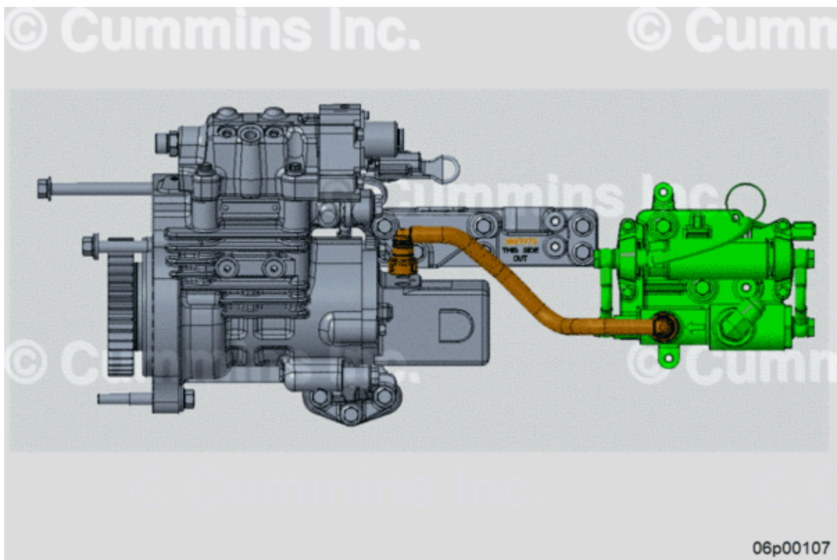
Figure 3, Existing Inlet Line Part Number 5440771 (Brown), Existing Gear Pump Part Number 4307482 (Gray), Priming Pump Part Number 3692468 (Green).
