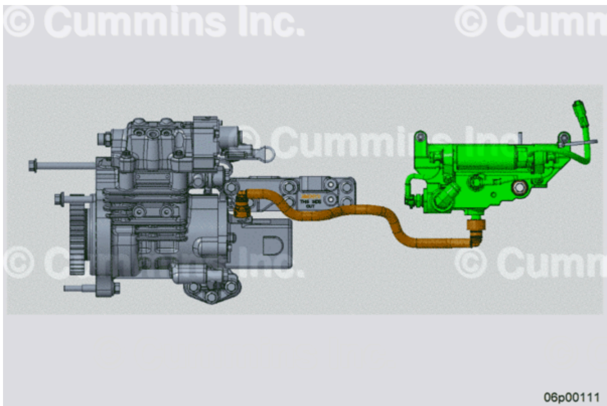
Figure 7, Existing Inlet Line Part Number 5440478 (Brown), Existing Gear Pump Part Number 4307482 (Gray), Priming Pump Part Number 3688896 (Green).
