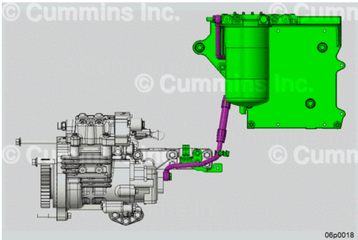
Figure 14, New Outlet Line Part Number 5575374 (Purple), New Gear Pump Part Number 5491782 (White), Fuel Filter Arrangement Part Number 3685850 (Green).
