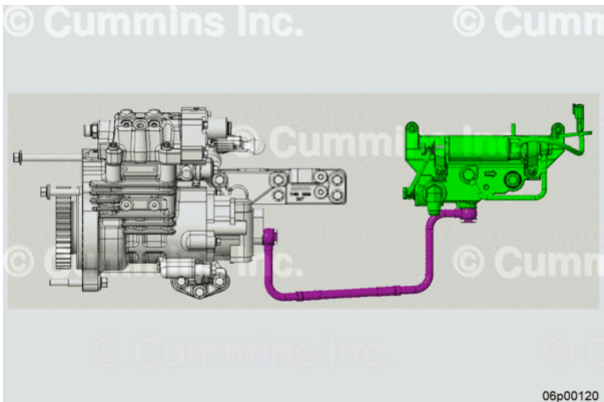
Figure 18, New Inlet Line Part Number 5566481 (Purple), New Gear Pump Part Number 5491782 (White), Priming Pump Part Number 5481052 (Green).
