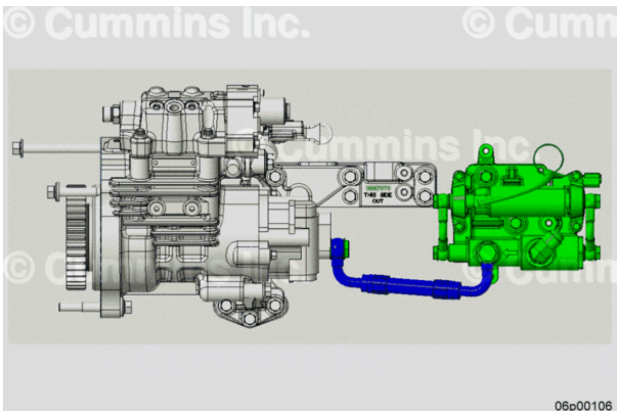
Figure 2, New Inlet Line Part Number 5575369 (Blue), New Gear Pump Part Number 5491782 (White), Priming Pump Part Number 3692468 (Green).
