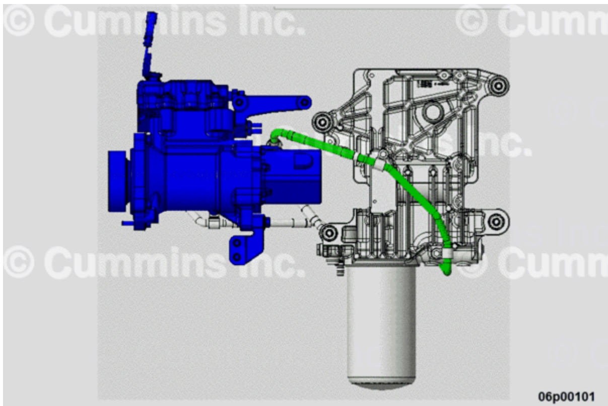
Figure 21, Existing Inlet Line, Part Number 2897186 (Green), Existing Gear Pump Part Number 5461704 (Blue), Fuel Filter Arrangement (White)
