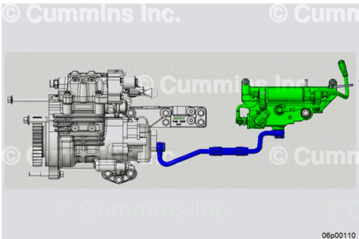
Figure 6, New Inlet Line Part Number 5575370 (Blue), New Gear Pump Part Number 5491782 (White), Priming Pump Part Number 3688896 (Green).
