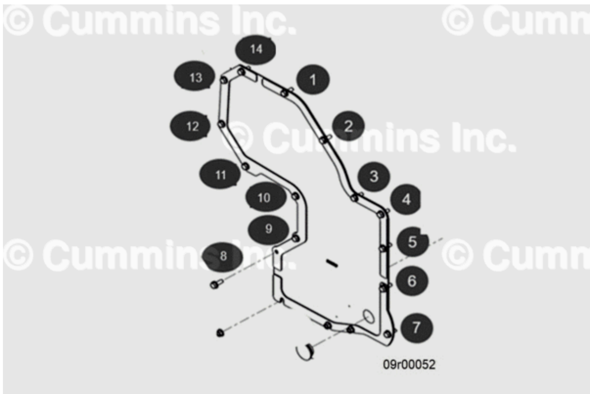
Figure 3, Gear Cover Capscrew Numbers.
