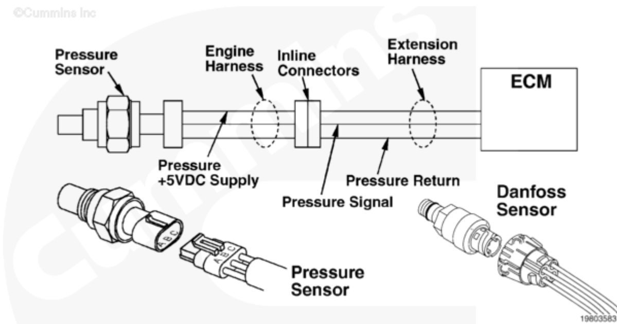
Fuel Timing Rail Pressure Sensor Circuit
