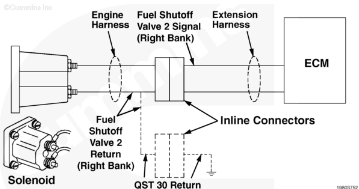
Fuel Shutoff Valve Solenoid Circuit
