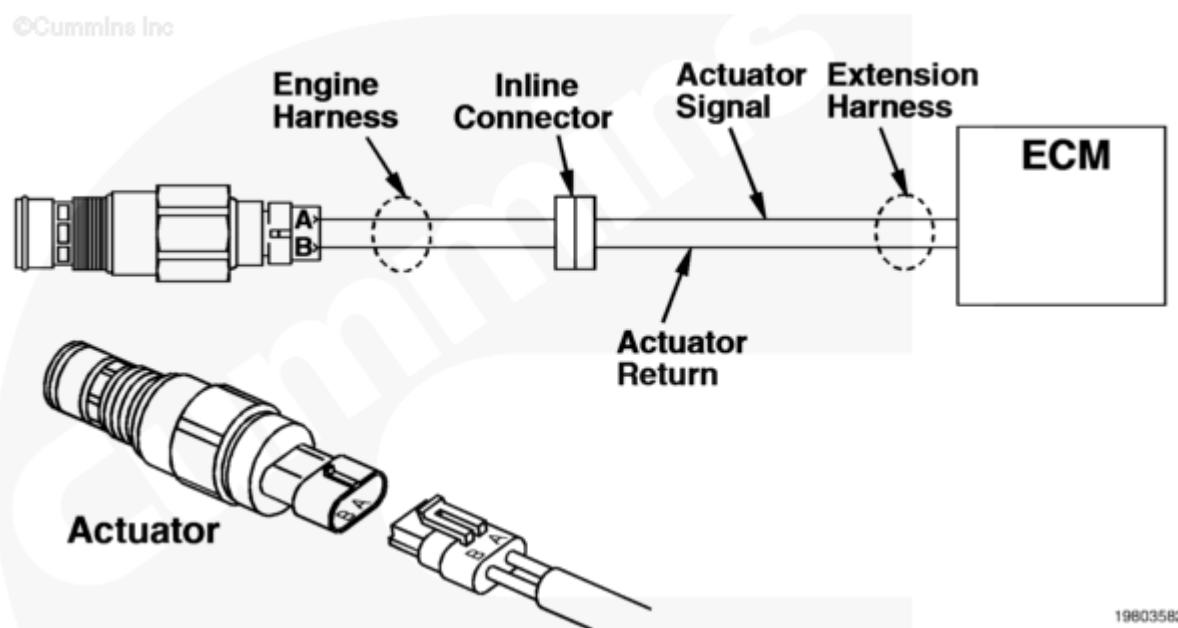
Timing Rail Number 1 Actuator Circuit
