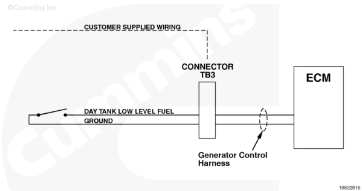
Day Tank Fuel Level Sensor Circuit
