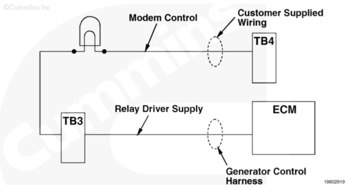
Modem Circuit
