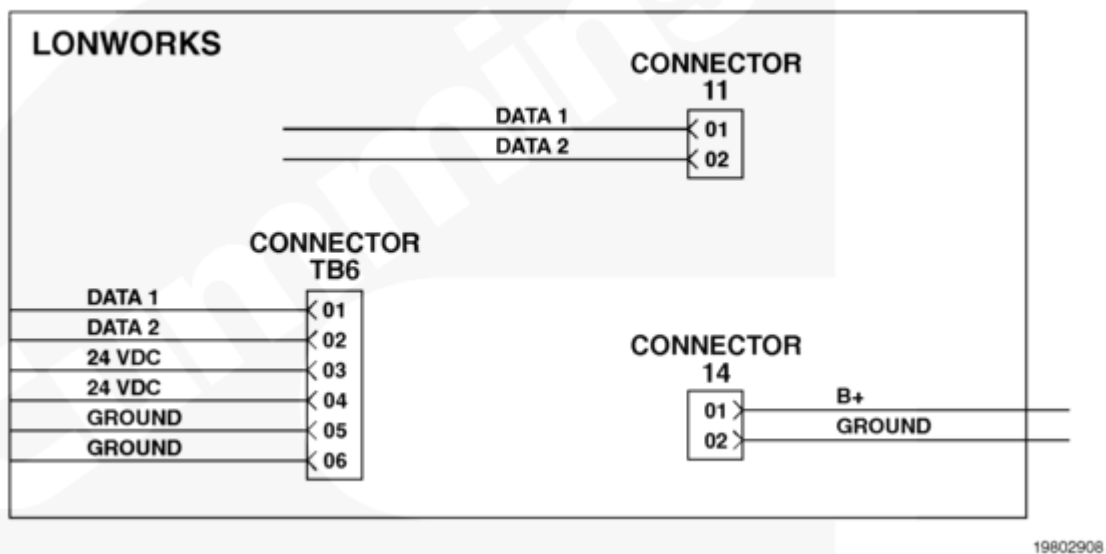
LonWorks Network Circuit
