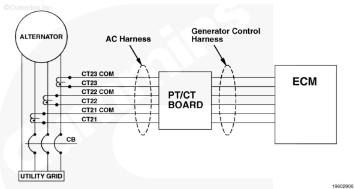
AC Output Current Circuit
