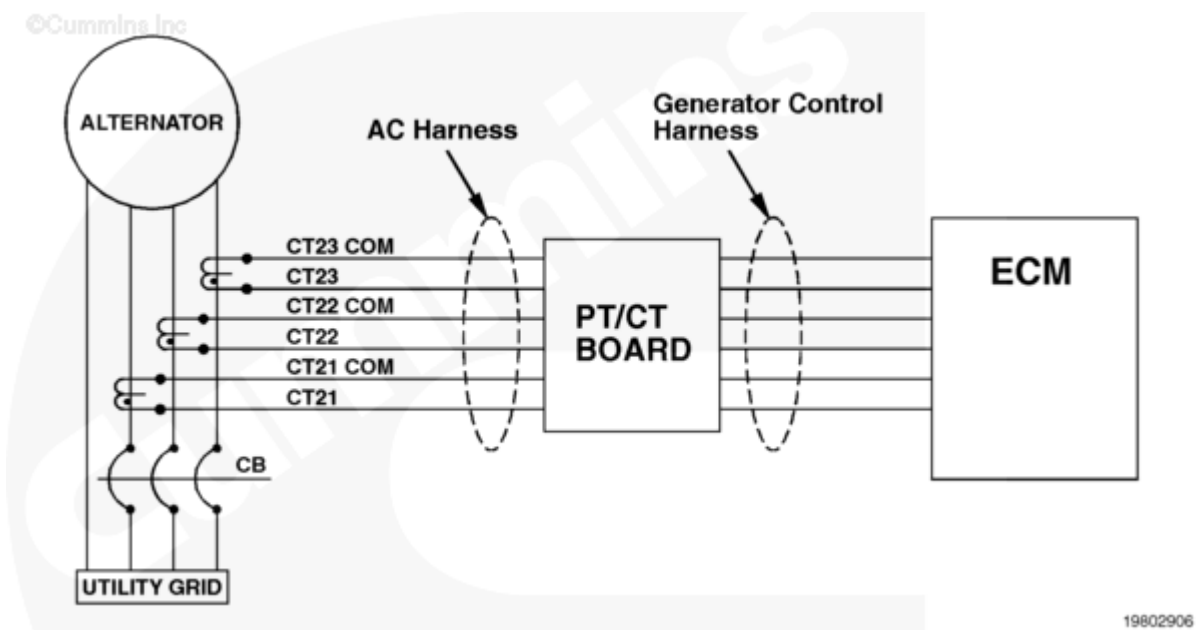
AC Output Current Circuit
