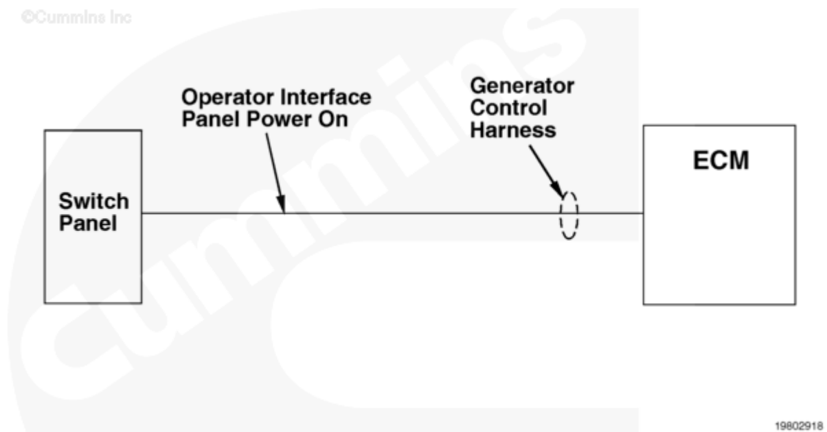
Operator Interface Panel Power Relay Driver Circuit
