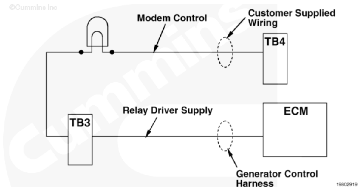
Modem Power Relay Driver Circuit
