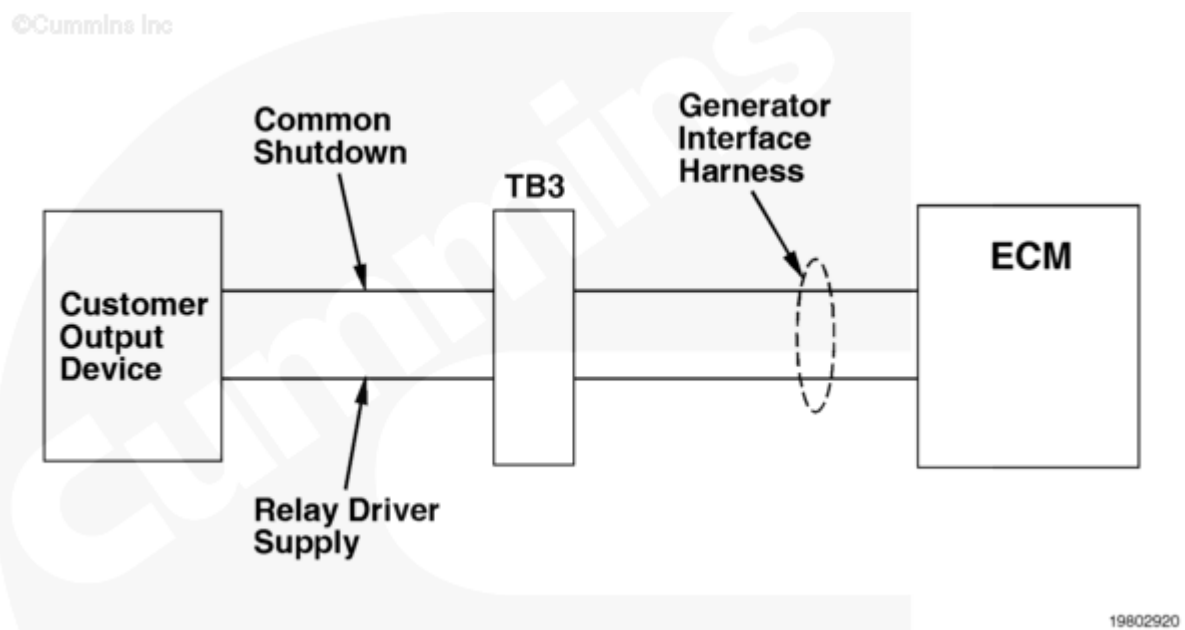
Common Shutdown Output Relay Driver Circuit
