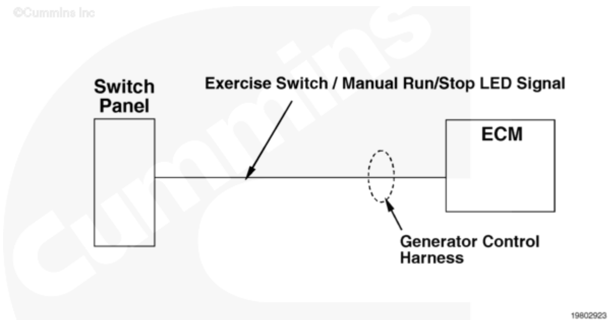
Exercise LED Driver Circuit
