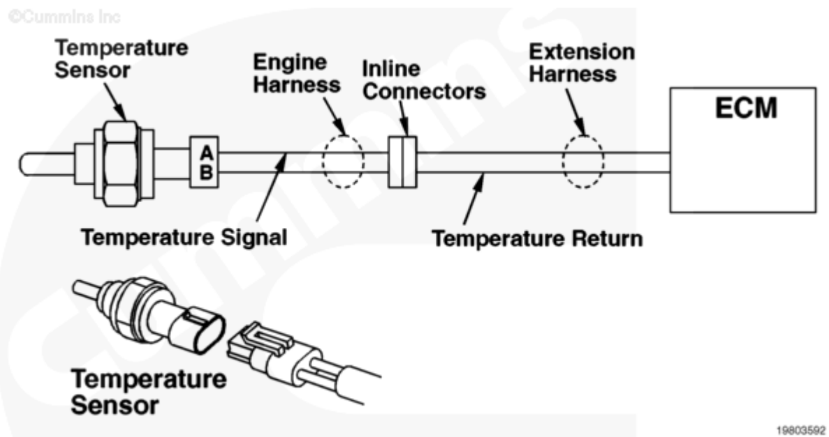
Aftercooler Water Inlet Temperature Sensor Circuit
