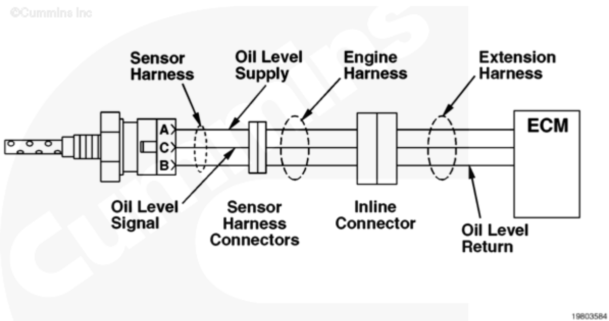
Oil Level Sensor Circuit
