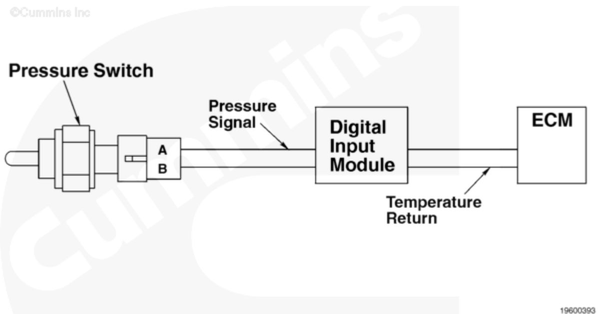
Engine Gear Box Oil Pressure Sensor Circuit
