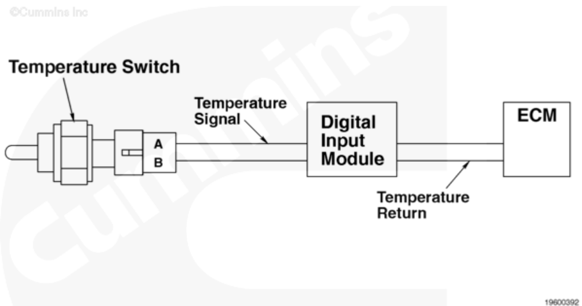
Engine Gear Box Oil Temperature Sensor Circuit
