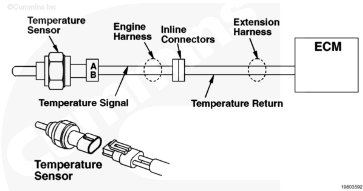
Fuel Temperature Sensor Circuit
