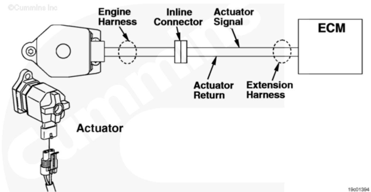
Fueling Actuator Number 1 Circuit
