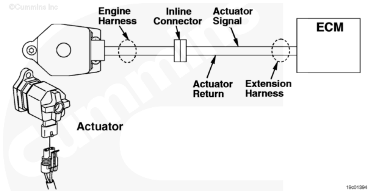
Timing Actuator Number 1 Circuit
