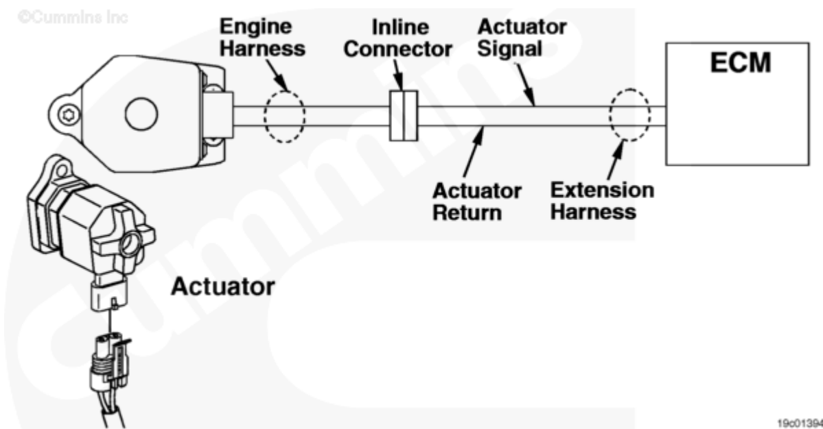
Fueling Actuator Number 2 Circuit
