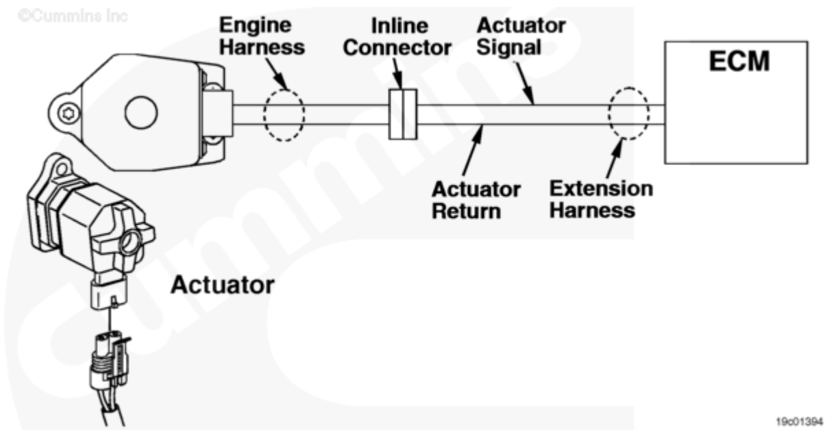
Timing Actuator Number 2 Circuit
