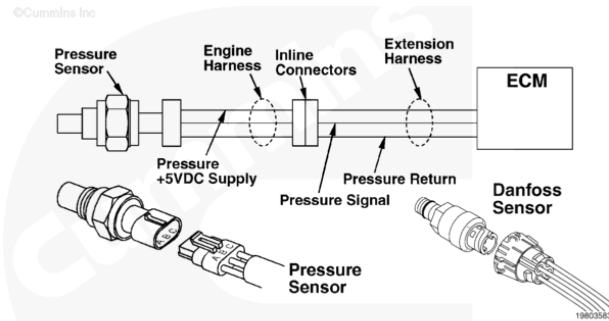
Fuel Rail Pressure Sensor Circuit
