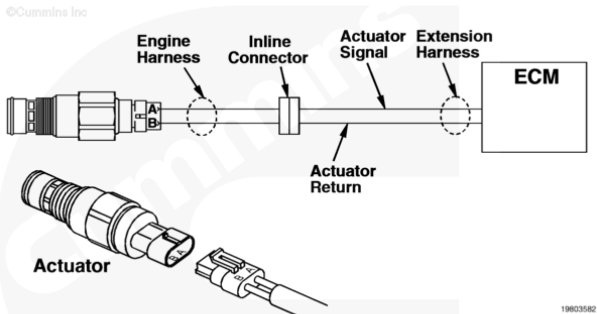
Fuel Rail Actuator Circuit
