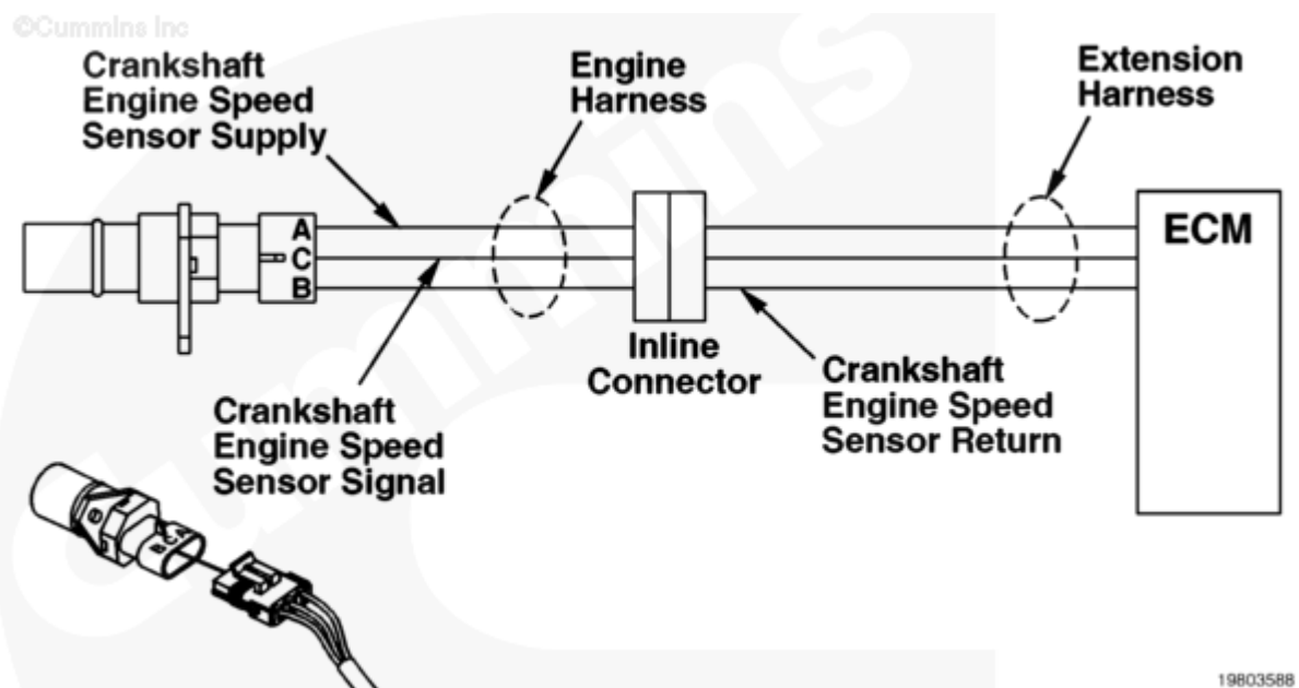
Crankshaft Engine Speed Sensor Circuit
