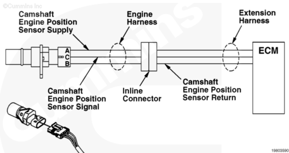
Camshaft Engine Position Sensor Circuit
