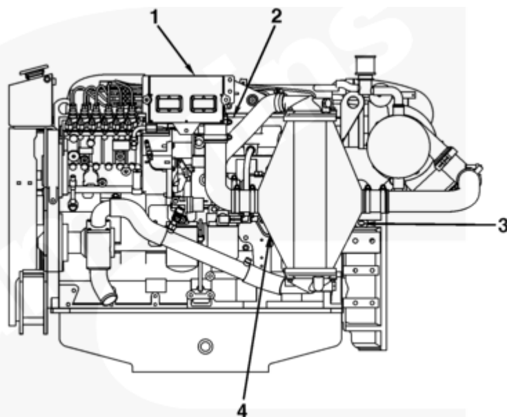
6CTA 480C Marine (Port View)
