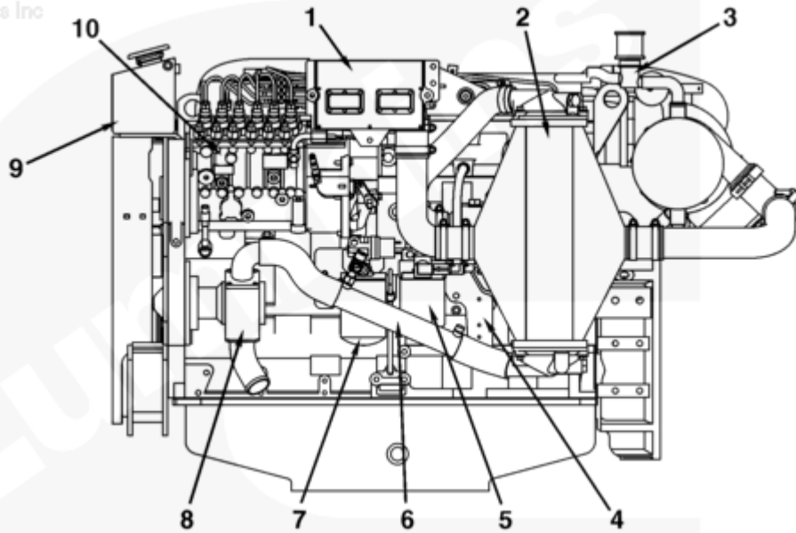
C8.3 Marine (Left View)
