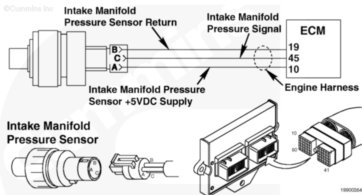
Intake Manifold Pressure Sensor Circuit
