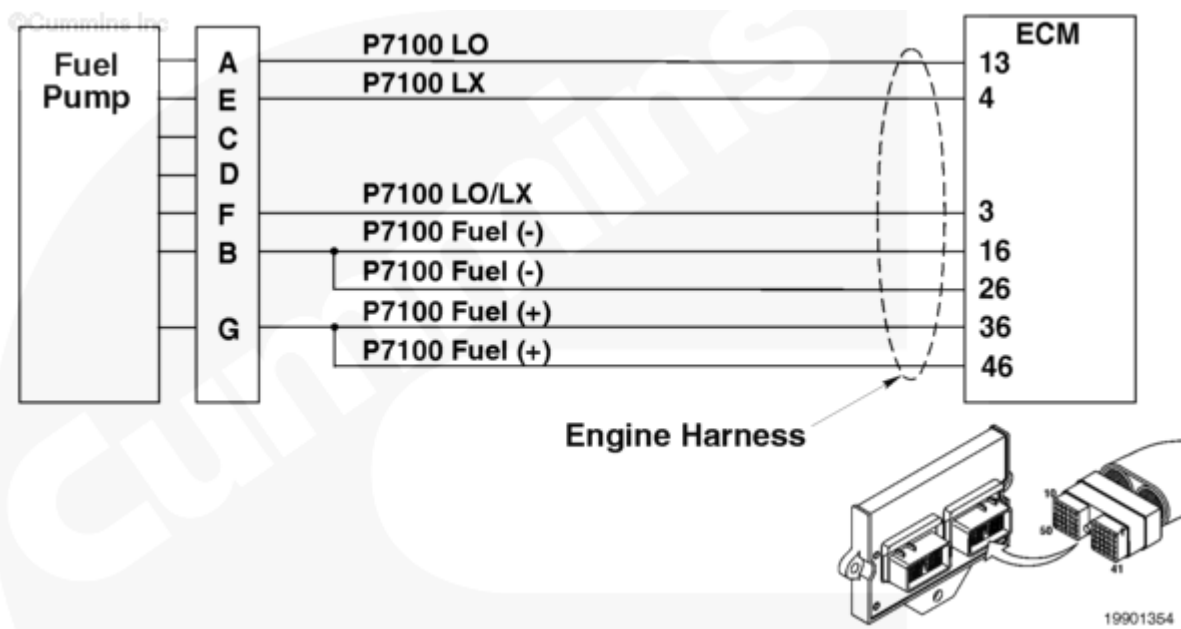
Rack Actuator Circuit
